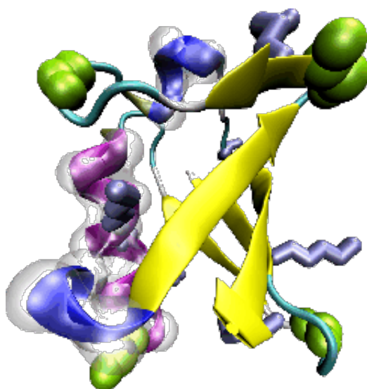
Figure 16: Example of a POV-Ray 3.6 (POV3) rendering.
