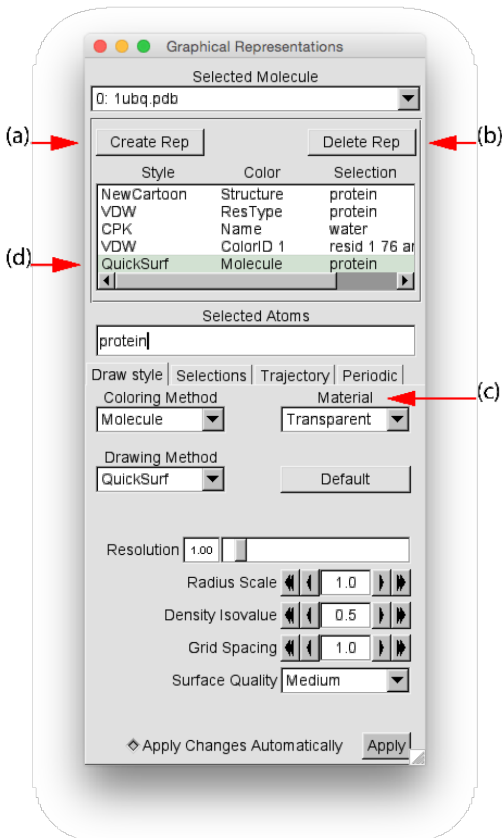
Figure 10: Multiple Representations of Ubiquitin.
