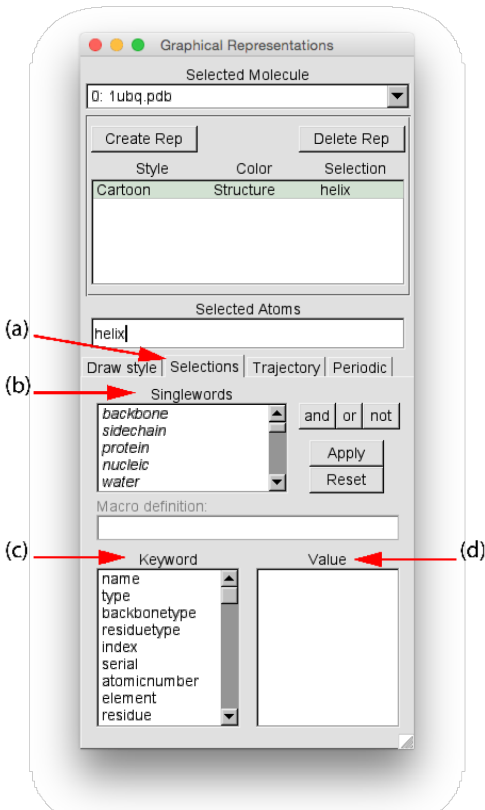
Figure 9: Graphical Representations window and the Selections tab.
