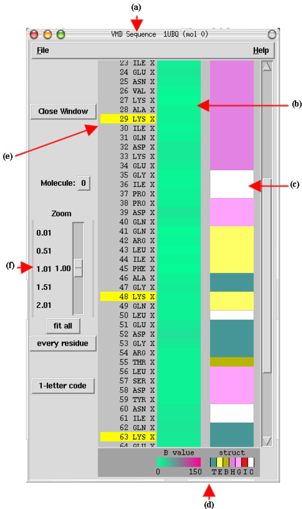
Figure 11: VMD Sequence window.
