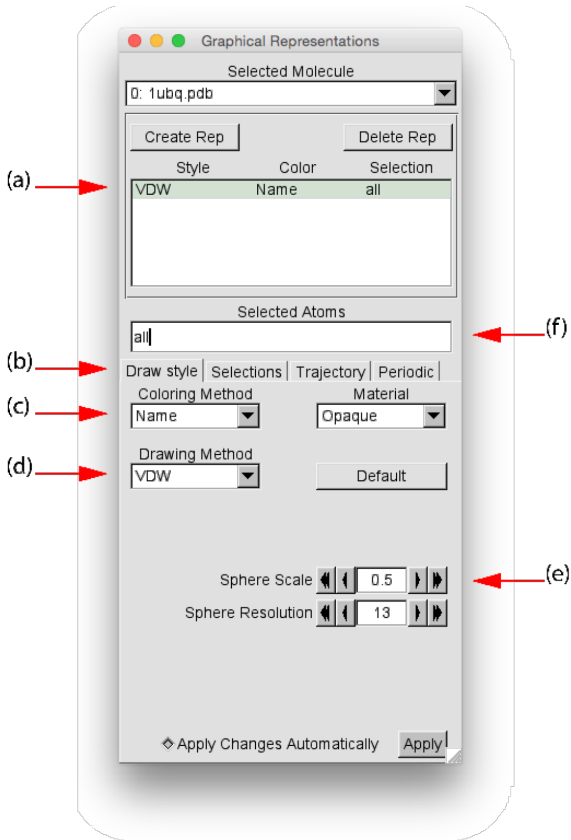
Figure 7: The Graphical Representations window.
