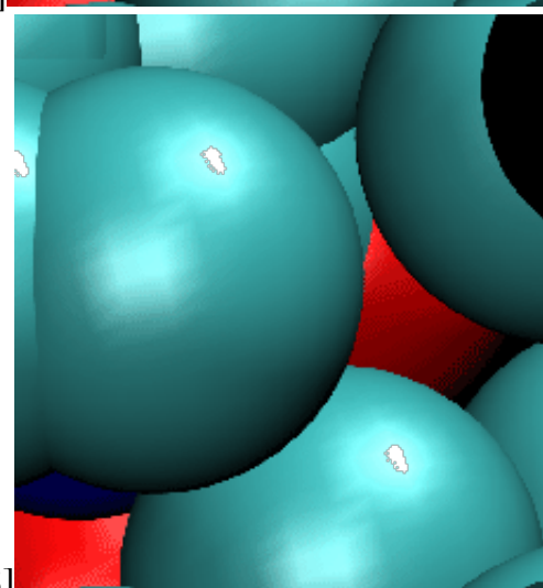
Figure 12: The effect of the resolution setting.
